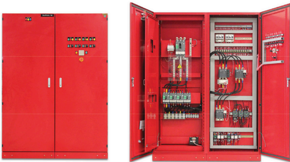
Tủ PCCC Fire Fighting Control Panel
